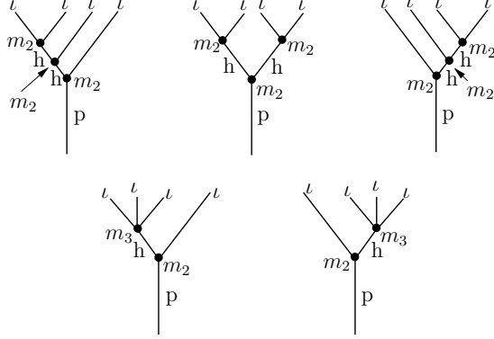
FIGURE 1. The full collection of rooted trees with 4 inputs specifying the multiplication m_4 described by Proposition 2.3.
