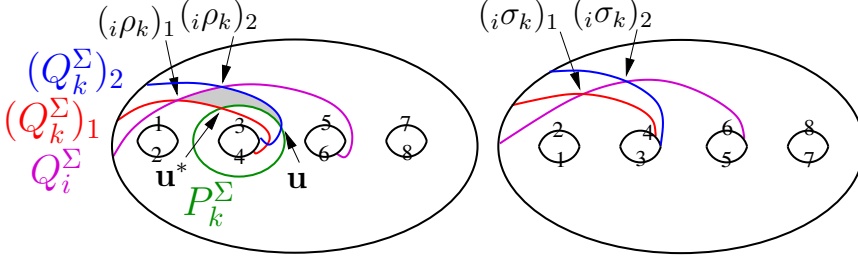
FIGURE 10. The above diagram verifies that
