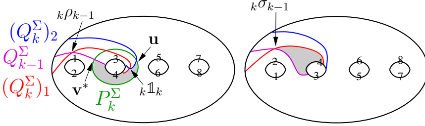
FIGURE 11. The above diagram verifies that
