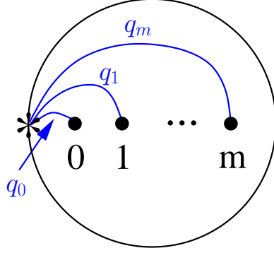
FIGURE 5. The basis \mathcal{Q} = \{q_0, \dots, q_m\}
