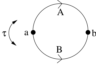
FIGURE 12. A \mathbb{Z}/2\mathbb{Z} -equivariant chain complex for S^1 .
